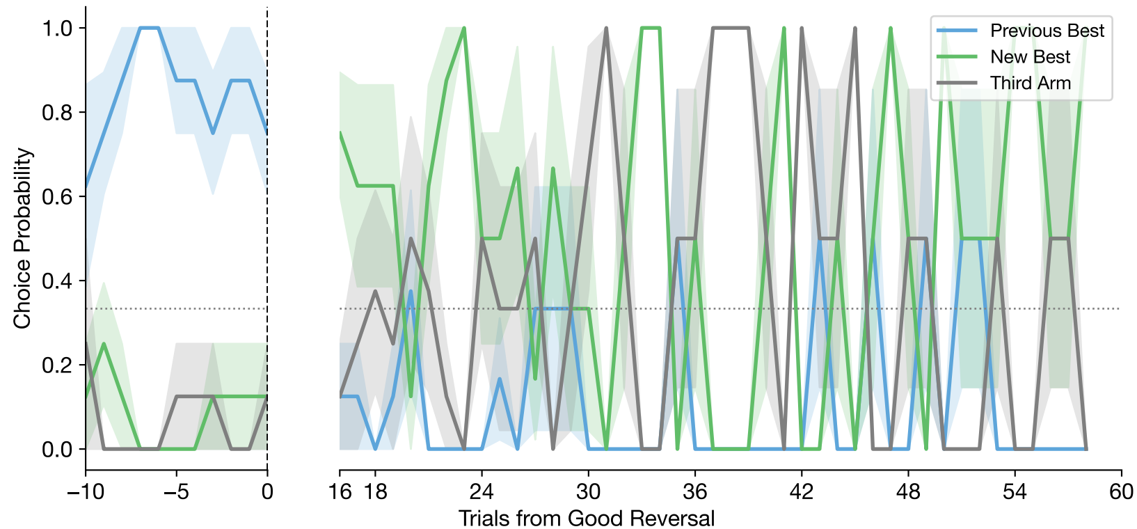
Good Reversal-Aligned Choices (mean \pm se across subjects | n=4 subjects, n=8 reversals) (Skipping first 15 trials post-reversal)
